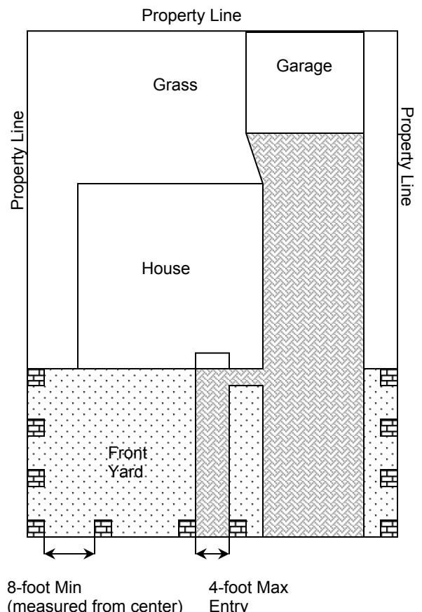
Example of Residential Site Plan- Non Corner Lot
