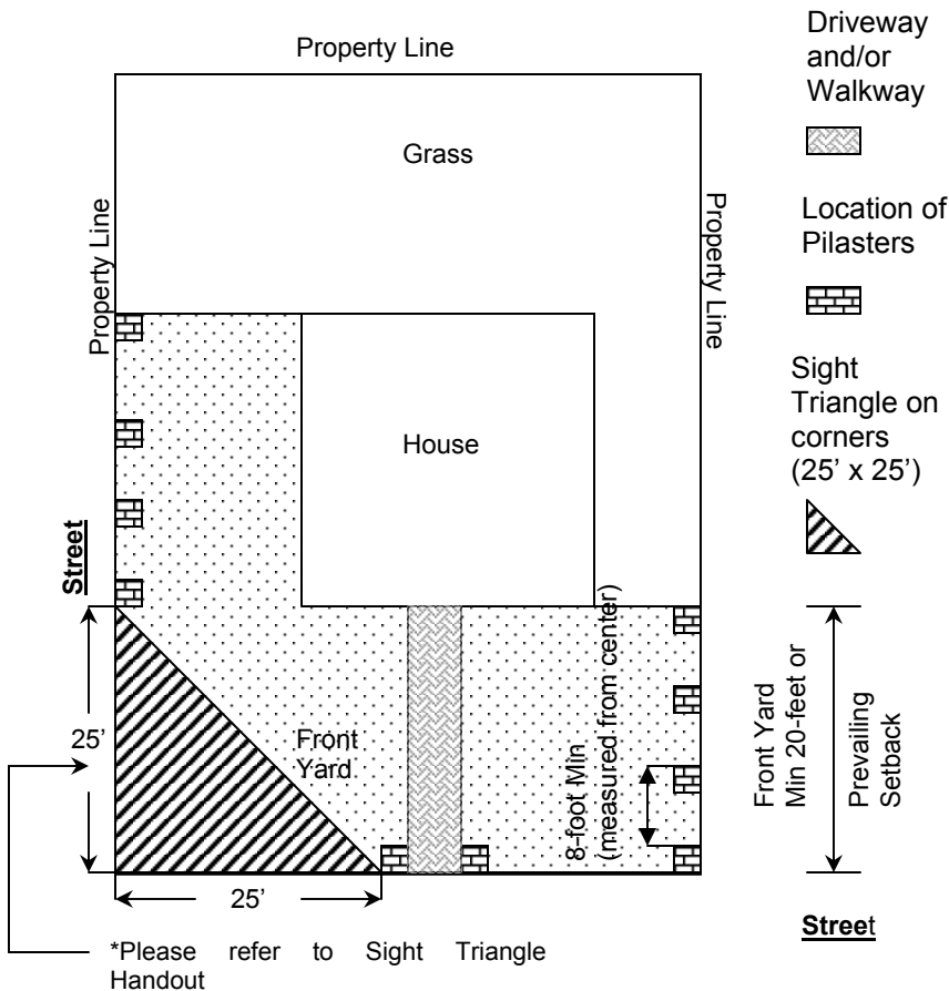
Example of Residential Site Plan- Corner Lot
