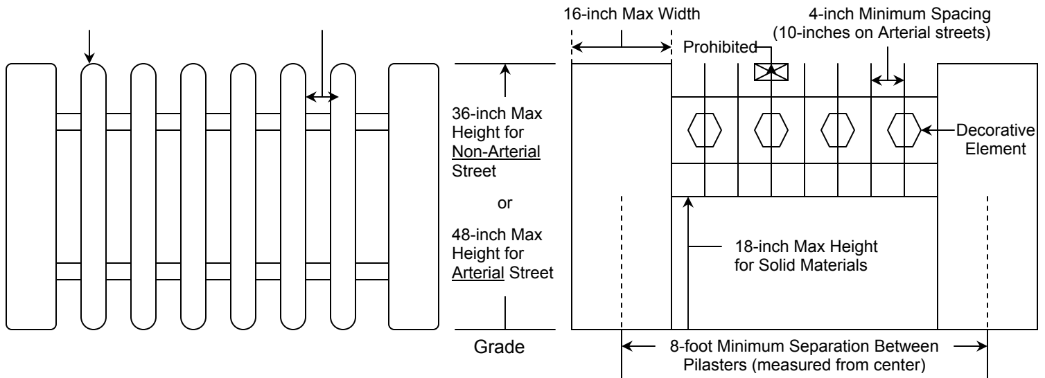
Example of Masonry Fence Design with Pilasters
